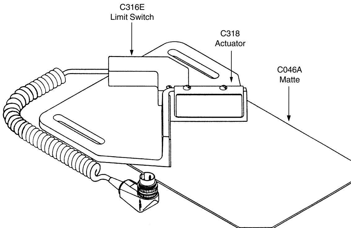
C325E Backstop Assembly
